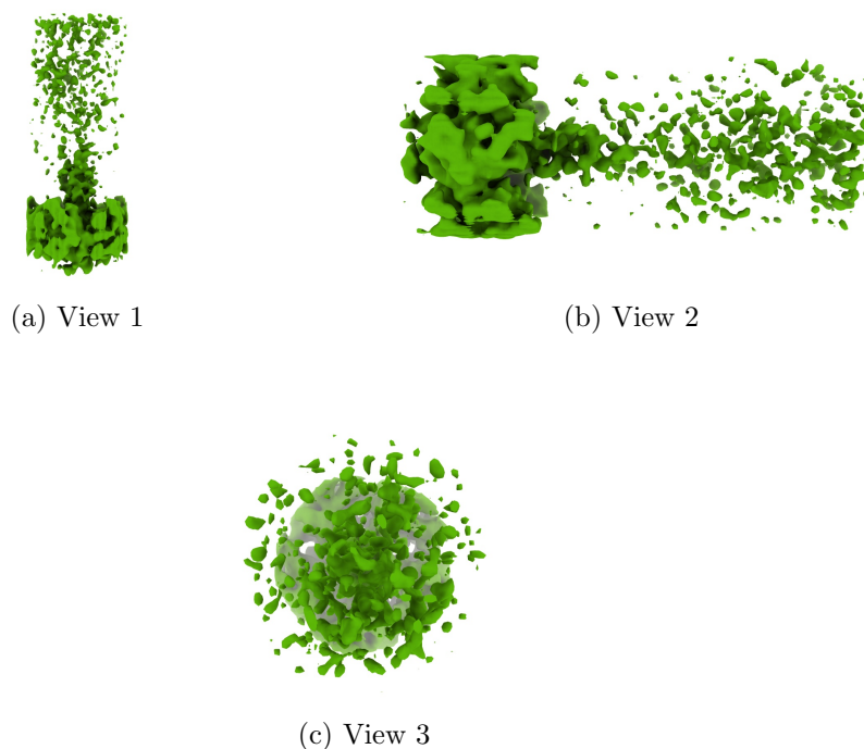
Figure 4: Isosurface at threshold=0.004260. Views generated by ChimeraX at a the following X, Y, Z angles: View 1 (0, -90, -90), View 2 (-90, 0, -90), View 3 (0, 0, 0).
