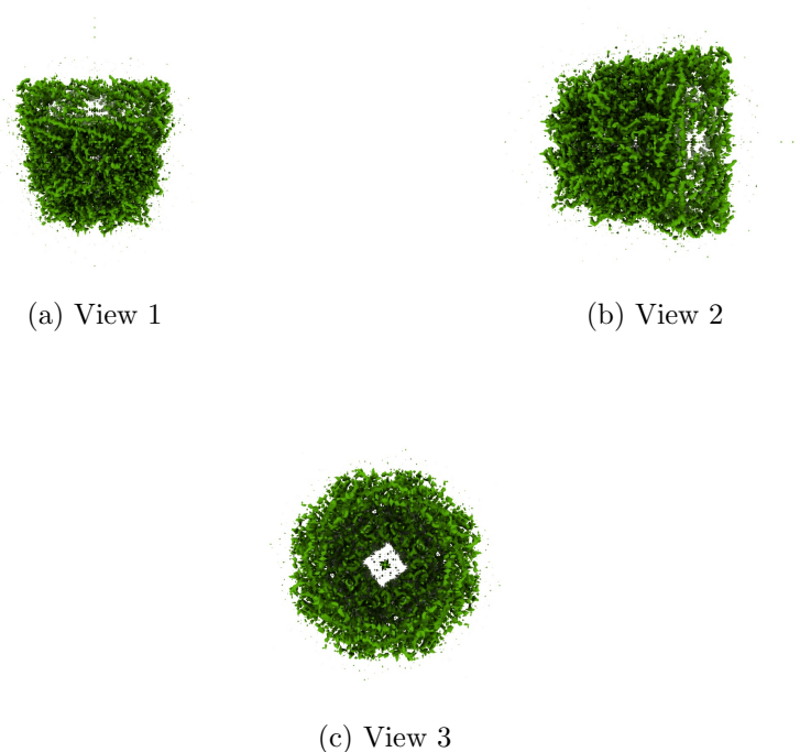
Figure 4: Isosurface at threshold=11.000000. Views generated by ChimeraX at a the following X, Y, Z angles: View 1 (0, -90, -90), View 2 (-90, 0, -90), View 3 (0, 0, 0).
