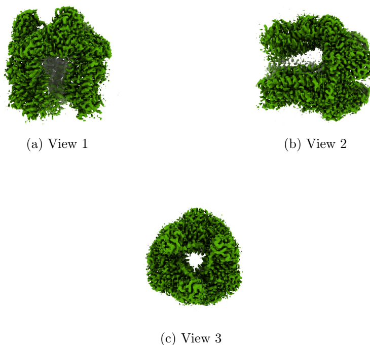
Figure 4: Isosurface at threshold=0.420000. Views generated by ChimeraX at a the following X, Y, Z angles: View 1 (0, -90, -90), View 2 (-90, 0, -90), View 3 (0, 0, 0).
