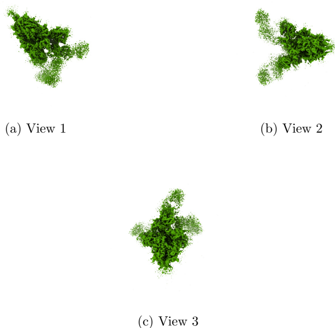
Figure 4: Isosurface at threshold=0.182000. Views generated by ChimeraX at a the following X, Y, Z angles: View 1 (0, -90, -90), View 2 (-90, 0, -90), View 3 (0, 0, 0).
