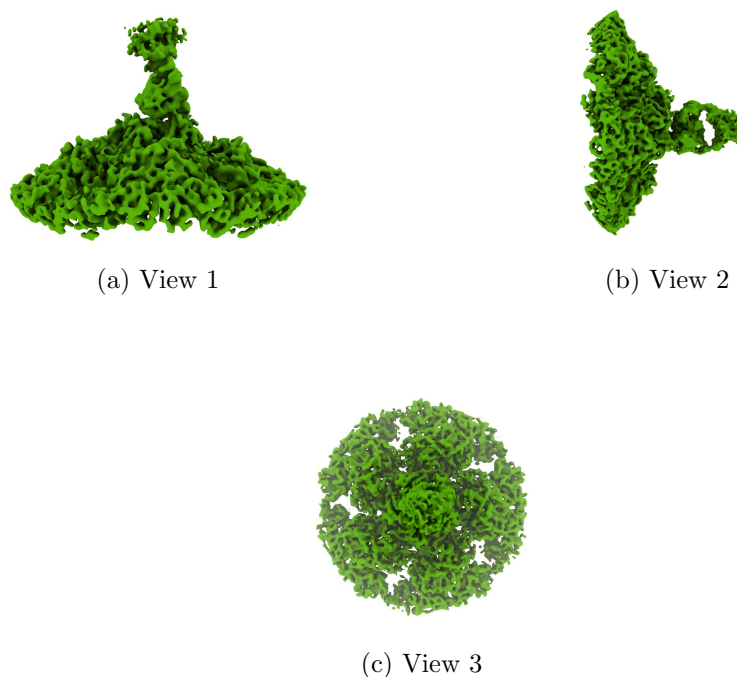
Figure 4: Isosurface at threshold=8.130000. Views generated by ChimeraX at a the following X, Y, Z angles: View 1 (0, -90, -90), View 2 (-90, 0, -90), View 3 (0, 0, 0).
