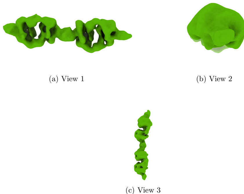
Figure 4: Isosurface at threshold=0.026000. Views generated by ChimeraX at a the following X, Y, Z angles: View 1 (0, -90, -90), View 2 (-90, 0, -90), View 3 (0, 0, 0).
