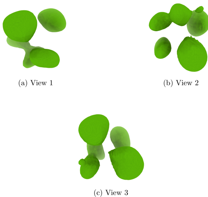
Figure 4: Isosurface at threshold=5.310000. Views generated by ChimeraX at a the following X, Y, Z angles: View 1 (0, -90, -90), View 2 (-90, 0, -90), View 3 (0, 0, 0).
