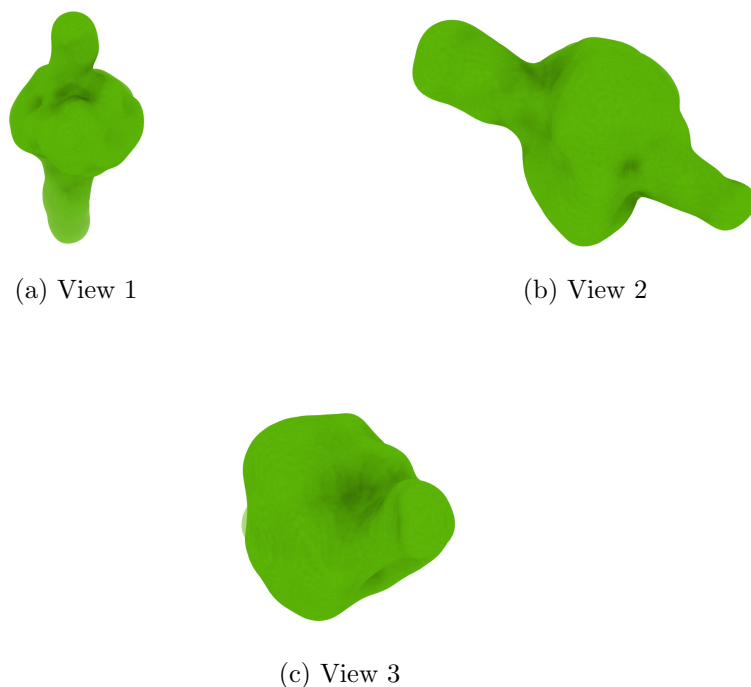
Figure 4: Isosurface at threshold=0.031700. Views generated by ChimeraX at a the following X, Y, Z angles: View 1 (0, -90, -90), View 2 (-90, 0, -90), View 3 (0, 0, 0).
