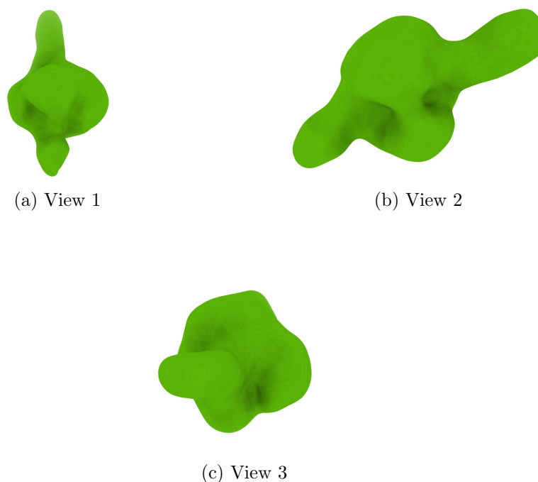
Figure 4: Isosurface at threshold=0.048400. Views generated by ChimeraX at a the following X, Y, Z angles: View 1 (0, -90, -90), View 2 (-90, 0, -90), View 3 (0, 0, 0).
