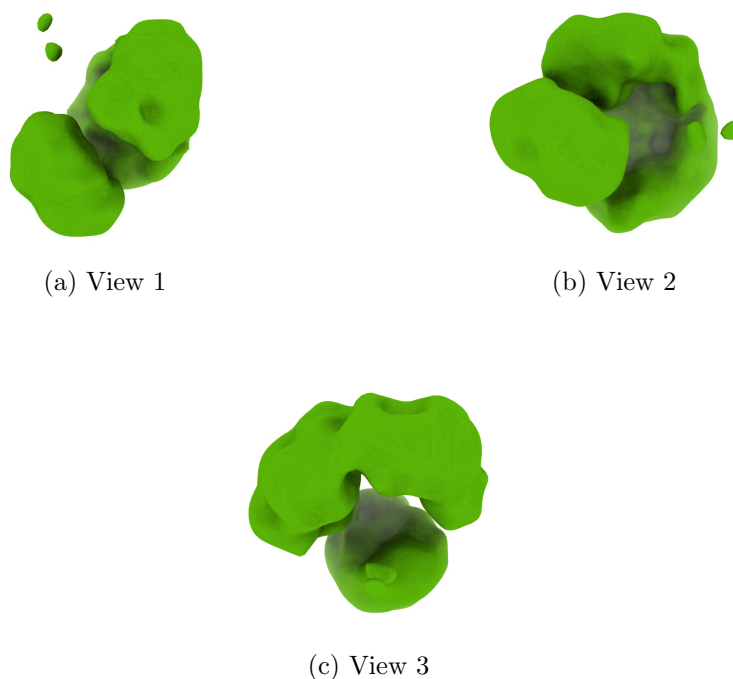
Figure 4: Isosurface at threshold=0.090800. Views generated by ChimeraX at a the following X, Y, Z angles: View 1 (0, -90, -90), View 2 (-90, 0, -90), View 3 (0, 0, 0).
