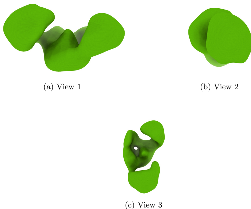
Figure 4: Isosurface at threshold=0.103000. Views generated by ChimeraX at a the following X, Y, Z angles: View 1 (0, -90, -90), View 2 (-90, 0, -90), View 3 (0, 0, 0).
