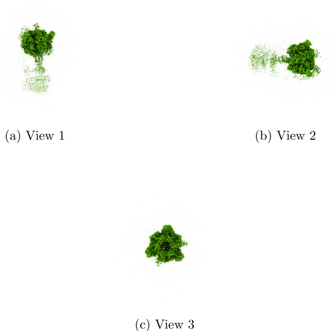
Figure 4: Isosurface at threshold=0.015500. Views generated by ChimeraX at a the following X, Y, Z angles: View 1 (0, -90, -90), View 2 (-90, 0, -90), View 3 (0, 0, 0).
