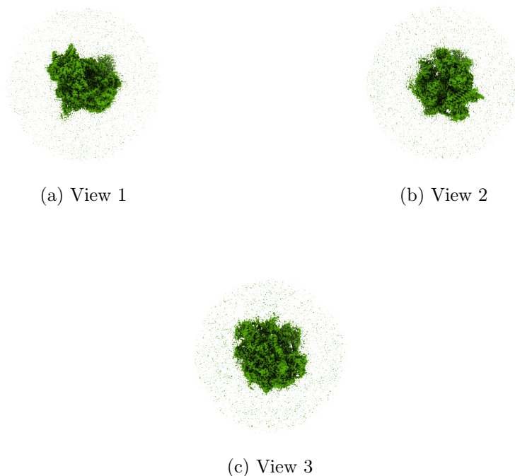
Figure 4: Isosurface at threshold=0.351000. Views generated by ChimeraX at a the following X, Y, Z angles: View 1 (0, -90, -90), View 2 (-90, 0, -90), View 3 (0, 0, 0).
