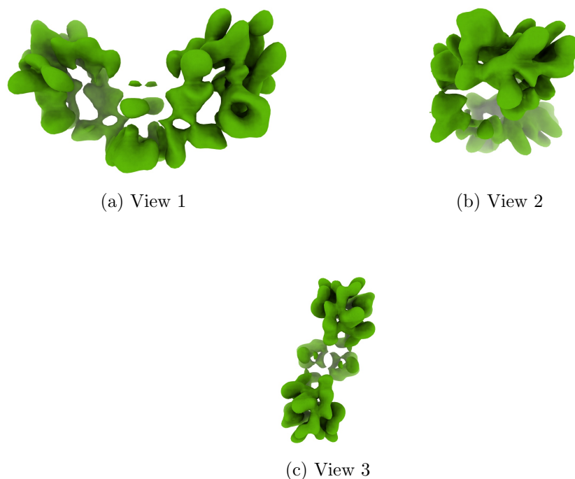
Figure 4: Isosurface at threshold=0.023100. Views generated by ChimeraX at a the following X, Y, Z angles: View 1 (0, -90, -90), View 2 (-90, 0, -90), View 3 (0, 0, 0).
