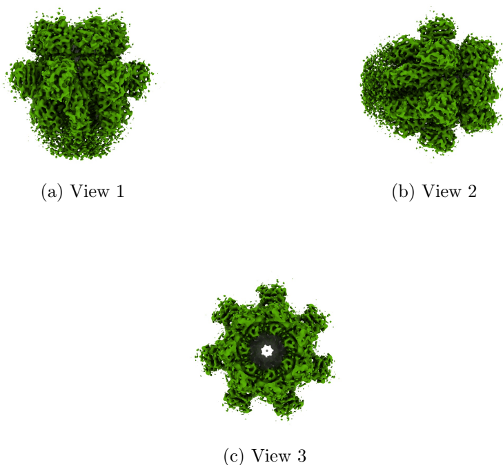
Figure 4: Isosurface at threshold=0.322000. Views generated by ChimeraX at a the following X, Y, Z angles: View 1 (0, -90, -90), View 2 (-90, 0, -90), View 3 (0, 0, 0).
