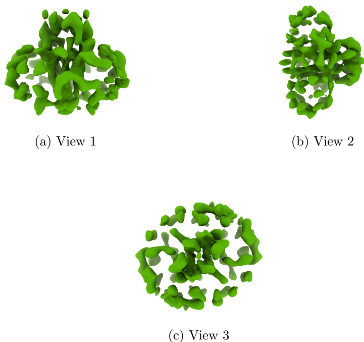
Figure 4: Isosurface at threshold=0.337000. Views generated by ChimeraX at a the following X, Y, Z angles: View 1 (0, -90, -90), View 2 (-90, 0, -90), View 3 (0, 0, 0).
