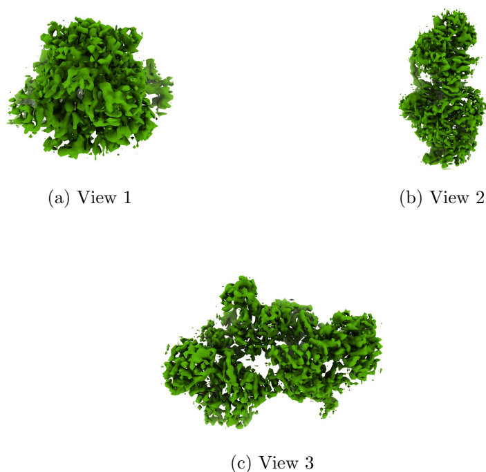
Figure 4: Isosurface at threshold=1.100000. Views generated by ChimeraX at a the following X, Y, Z angles: View 1 (0, -90, -90), View 2 (-90, 0, -90), View 3 (0, 0, 0).
