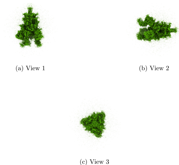
Figure 4: Isosurface at threshold=0.192000. Views generated by ChimeraX at a the following X, Y, Z angles: View 1 (0, -90, -90), View 2 (-90, 0, -90), View 3 (0, 0, 0).
