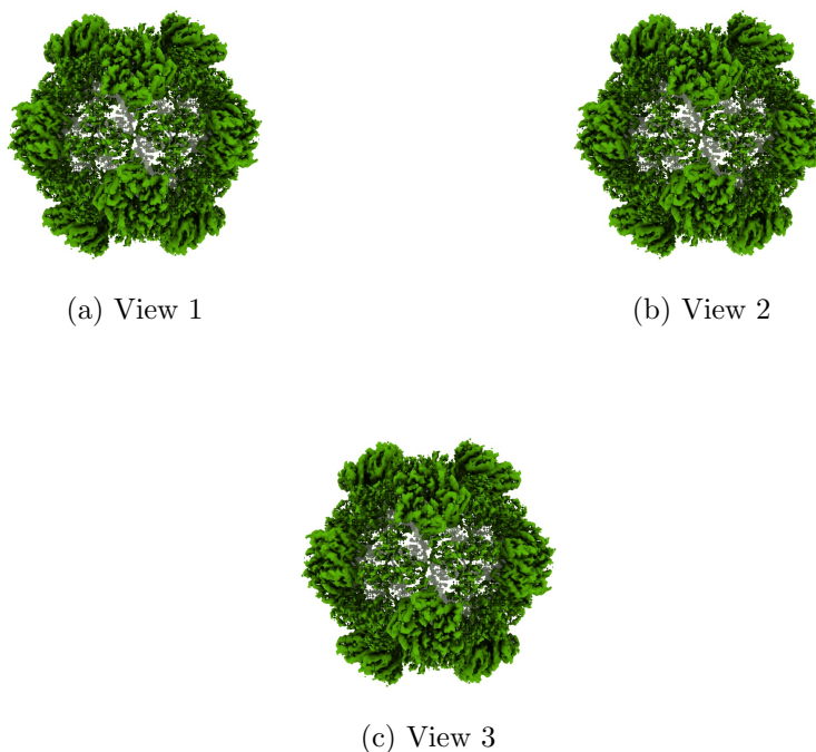
Figure 4: Isosurface at threshold=0.725000. Views generated by ChimeraX at a the following X, Y, Z angles: View 1 (0, -90, -90), View 2 (-90, 0, -90), View 3 (0, 0, 0).
