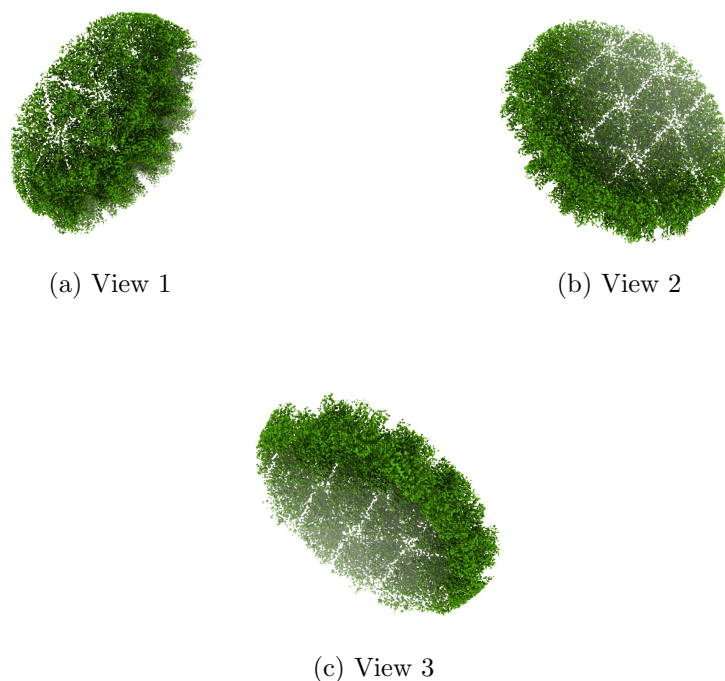
Figure 4: Isosurface at threshold=0.060000. Views generated by ChimeraX at a the following X, Y, Z angles: View 1 (0, -90, -90), View 2 (-90, 0, -90), View 3 (0, 0, 0).
