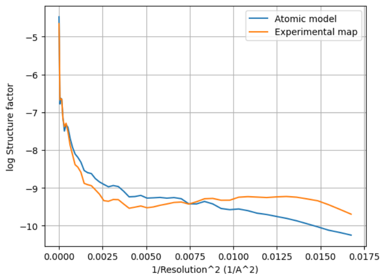
Figure 15: Guinier plot of the atom model and experimental map. The X-axis is the square of the inverse of the resolution in Å.
