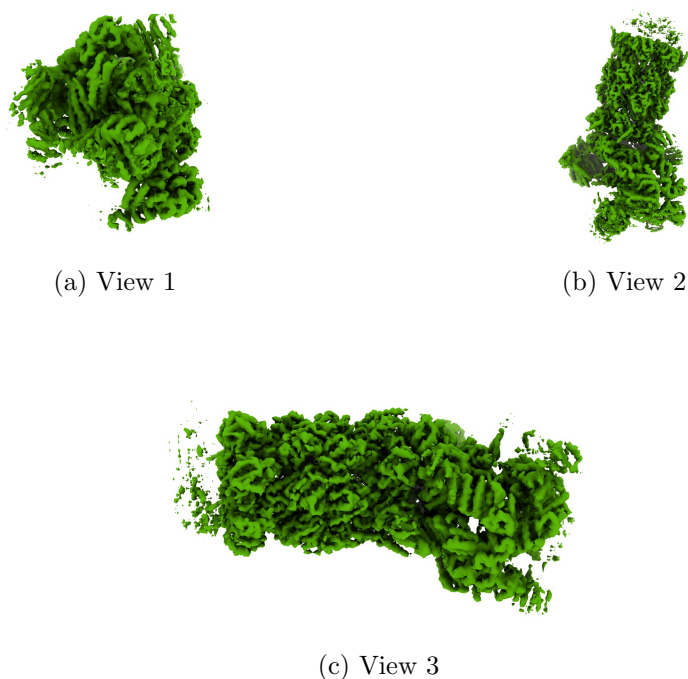
Figure 4: Isosurface at threshold=0.028000. Views generated by ChimeraX at a the following X, Y, Z angles: View 1 (0, -90, -90), View 2 (-90, 0, -90), View 3 (0, 0, 0).
