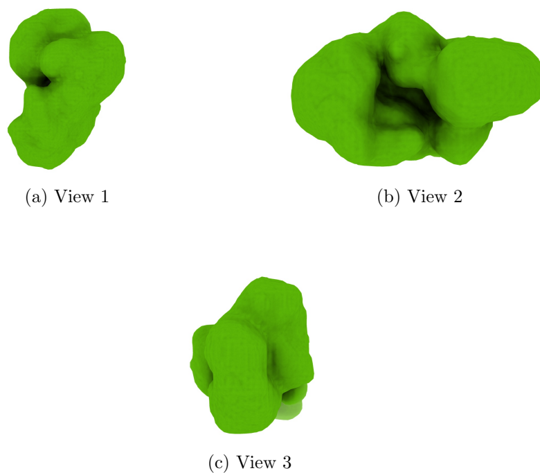
Figure 4: Isosurface at threshold=0.348000. Views generated by ChimeraX at a the following X, Y, Z angles: View 1 (0, -90, -90), View 2 (-90, 0, -90), View 3 (0, 0, 0).
