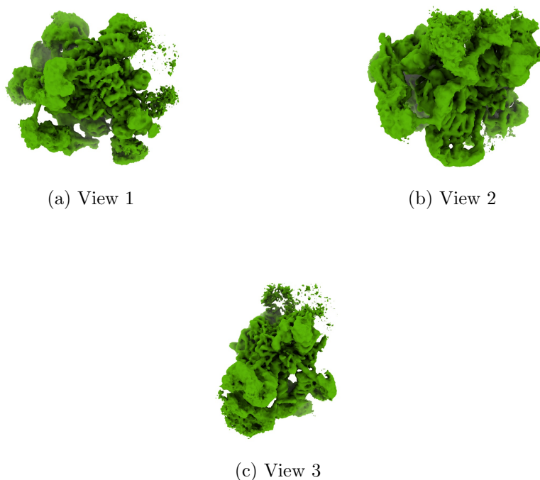
Figure 4: Isosurface at threshold=0.360000. Views generated by ChimeraX at a the following X, Y, Z angles: View 1 (0, -90, -90), View 2 (-90, 0, -90), View 3 (0, 0, 0).
