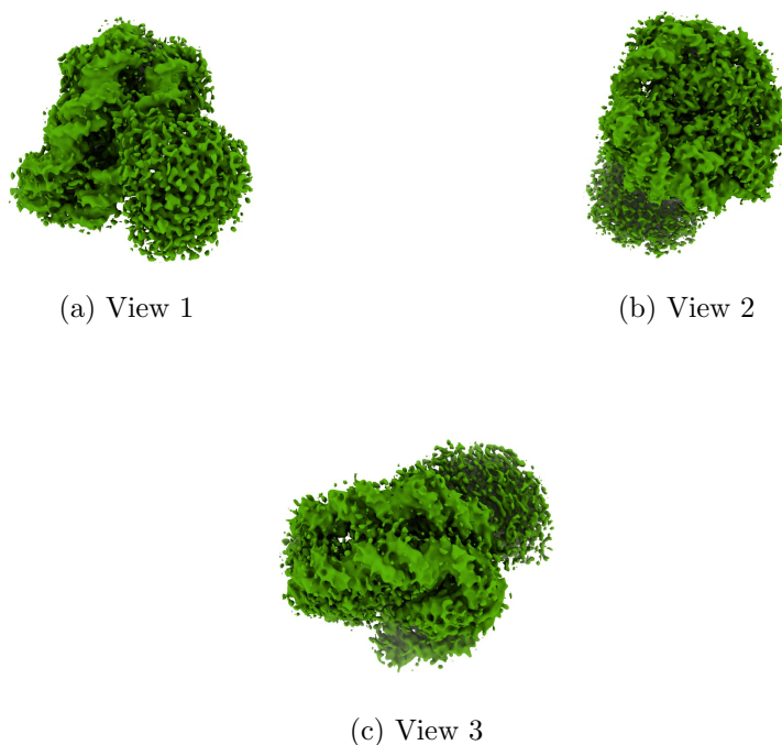
Figure 4: Isosurface at threshold=0.008900. Views generated by ChimeraX at a the following X, Y, Z angles: View 1 (0, -90, -90), View 2 (-90, 0, -90), View 3 (0, 0, 0).
