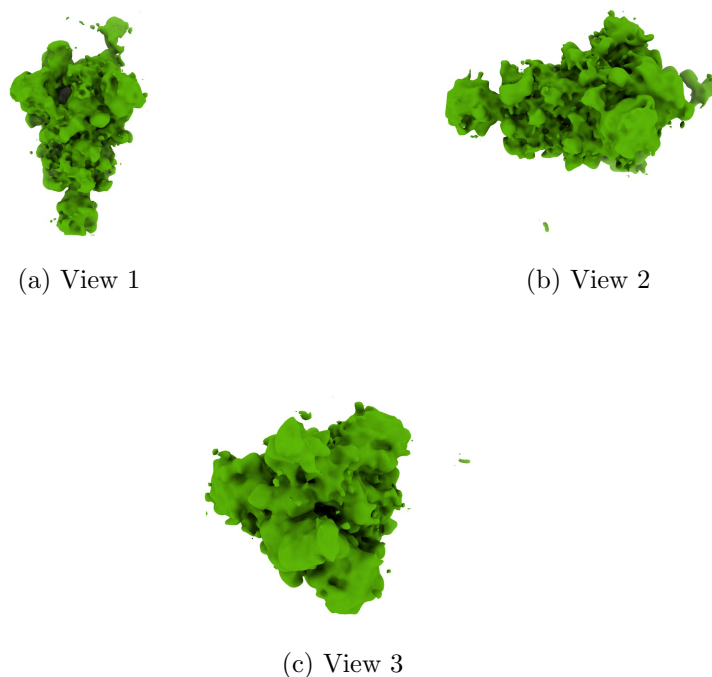
Figure 4: Isosurface at threshold=0.001340. Views generated by ChimeraX at a the following X, Y, Z angles: View 1 (0, -90, -90), View 2 (-90, 0, -90), View 3 (0, 0, 0).
