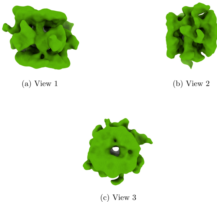
Figure 4: Isosurface at threshold=0.021700. Views generated by ChimeraX at a the following X, Y, Z angles: View 1 (0, -90, -90), View 2 (-90, 0, -90), View 3 (0, 0, 0).
