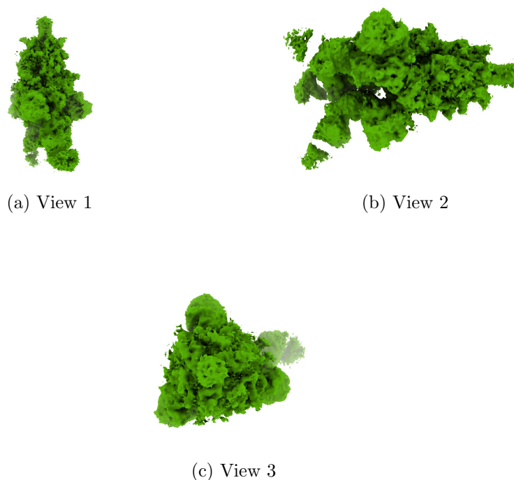
Figure 4: Isosurface at threshold=0.219000. Views generated by ChimeraX at a the following X, Y, Z angles: View 1 (0, -90, -90), View 2 (-90, 0, -90), View 3 (0, 0, 0).
