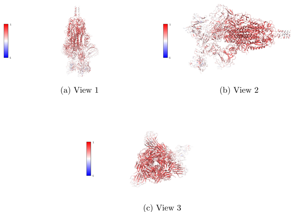
Figure 17: Atomic model colored by MapQ Views generated by ChimeraX at the following X, Y, Z angles: View 1 (0, -90, -90), View 2 (-90, 0, -90), View 3 (0, 0, 0).
