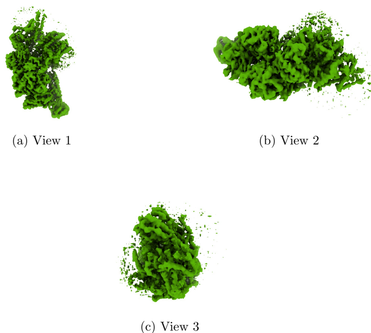
Figure 4: Isosurface at threshold=0.520000. Views generated by ChimeraX at a the following X, Y, Z angles: View 1 (0, -90, -90), View 2 (-90, 0, -90), View 3 (0, 0, 0).
