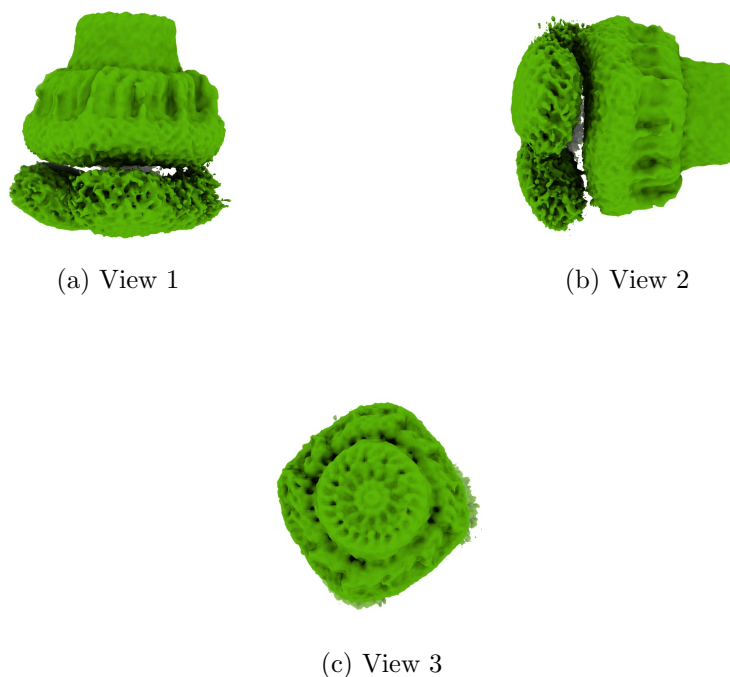
Figure 4: Isosurface at threshold=0.005560. Views generated by ChimeraX at a the following X, Y, Z angles: View 1 (0, -90, -90), View 2 (-90, 0, -90), View 3 (0, 0, 0).
