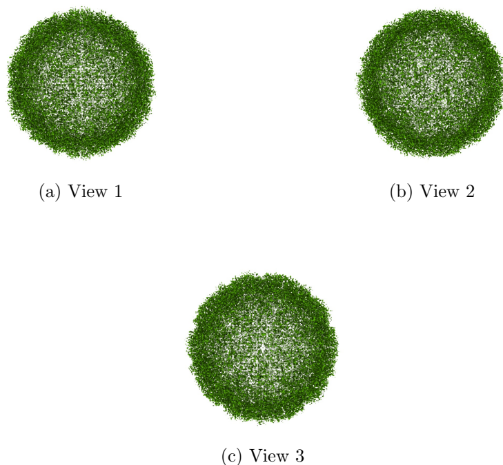
Figure 4: Isosurface at threshold=0.064900. Views generated by ChimeraX at a the following X, Y, Z angles: View 1 (0, -90, -90), View 2 (-90, 0, -90), View 3 (0, 0, 0).
