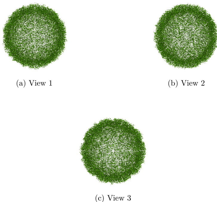
Figure 4: Isosurface at threshold=0.040200. Views generated by ChimeraX at a the following X, Y, Z angles: View 1 (0, -90, -90), View 2 (-90, 0, -90), View 3 (0, 0, 0).
