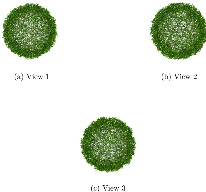
Figure 4: Isosurface at threshold=0.022800. Views generated by ChimeraX at a the following X, Y, Z angles: View 1 (0, -90, -90), View 2 (-90, 0, -90), View 3 (0, 0, 0).
