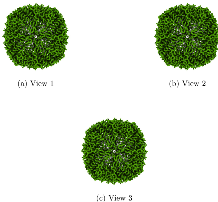
Figure 4: Isosurface at threshold=0.044300. Views generated by ChimeraX at a the following X, Y, Z angles: View 1 (0, -90, -90), View 2 (-90, 0, -90), View 3 (0, 0, 0).
