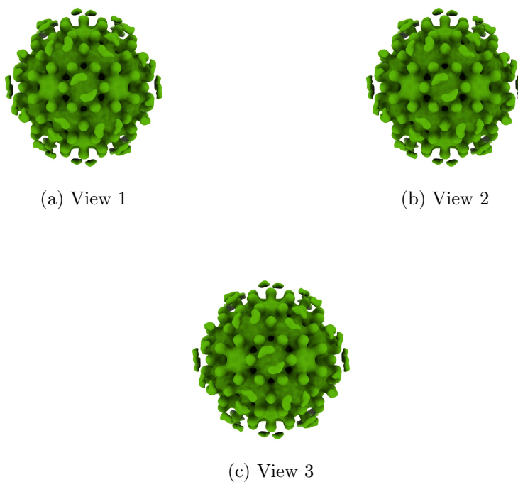
Figure 4: Isosurface at threshold=212.000000. Views generated by ChimeraX at a the following X, Y, Z angles: View 1 (0, -90, -90), View 2 (-90, 0, -90), View 3 (0, 0, 0).
