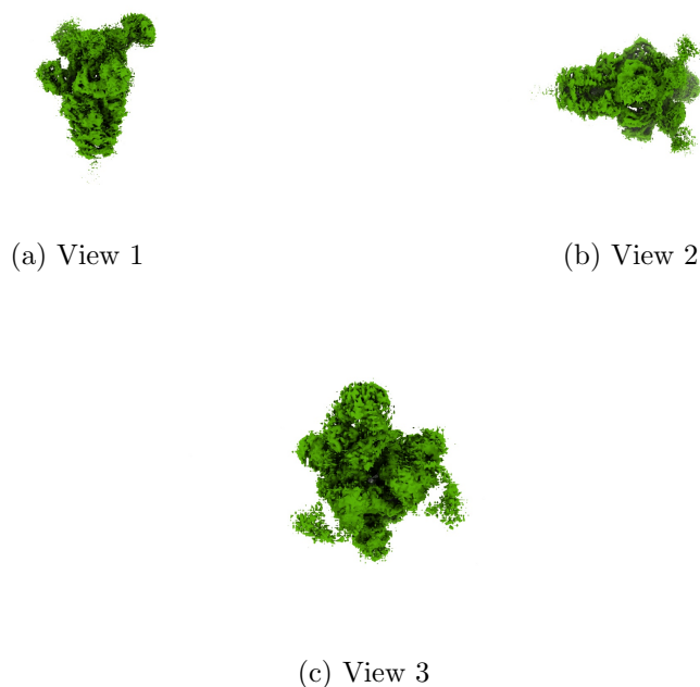
Figure 4: Isosurface at threshold=0.230000. Views generated by ChimeraX at a the following X, Y, Z angles: View 1 (0, -90, -90), View 2 (-90, 0, -90), View 3 (0, 0, 0).
