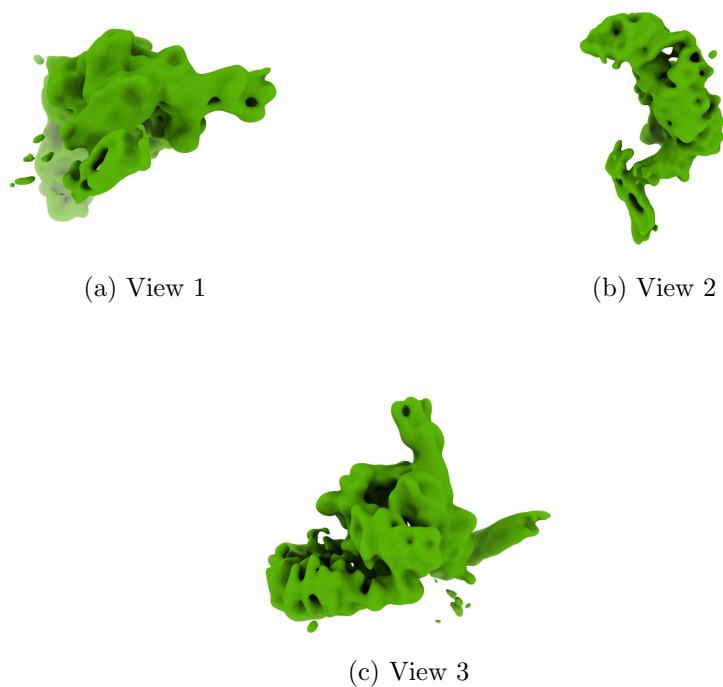
Figure 4: Isosurface at threshold=0.052600. Views generated by ChimeraX at a the following X, Y, Z angles: View 1 (0, -90, -90), View 2 (-90, 0, -90), View 3 (0, 0, 0).
