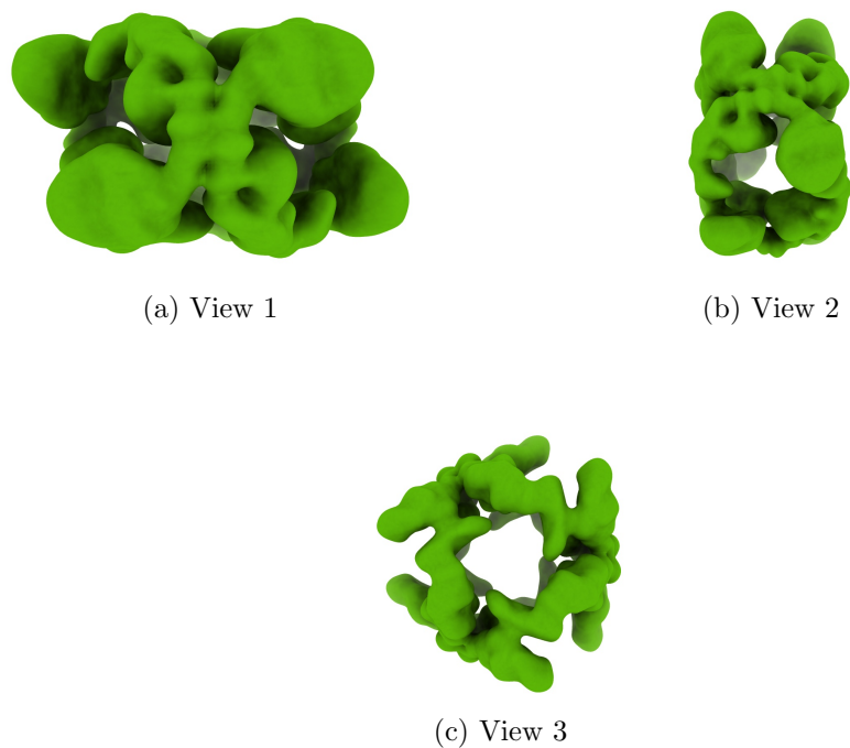
Figure 4: Isosurface at threshold=0.019200. Views generated by ChimeraX at a the following X, Y, Z angles: View 1 (0, -90, -90), View 2 (-90, 0, -90), View 3 (0, 0, 0).
