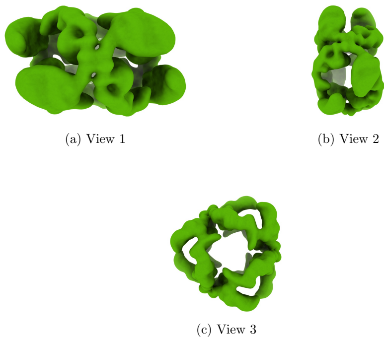
Figure 4: Isosurface at threshold=0.029300. Views generated by ChimeraX at a the following X, Y, Z angles: View 1 (0, -90, -90), View 2 (-90, 0, -90), View 3 (0, 0, 0).
