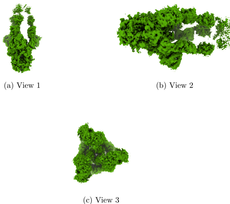
Figure 4: Isosurface at threshold=0.006770. Views generated by ChimeraX at a the following X, Y, Z angles: View 1 (0, -90, -90), View 2 (-90, 0, -90), View 3 (0, 0, 0).
