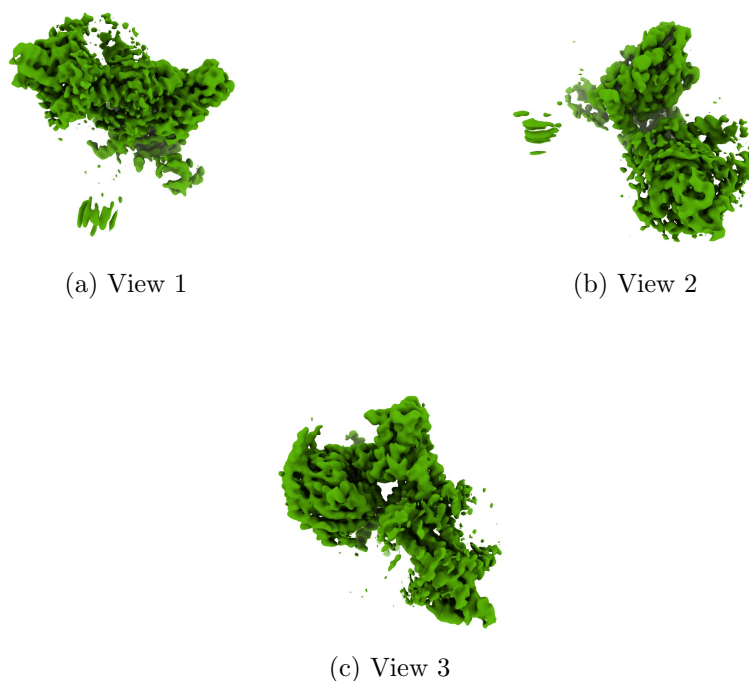
Figure 4: Isosurface at threshold=0.296000. Views generated by ChimeraX at a the following X, Y, Z angles: View 1 (0, -90, -90), View 2 (-90, 0, -90), View 3 (0, 0, 0).
