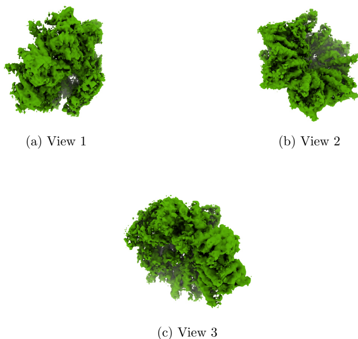
Figure 4: Isosurface at threshold=0.005510. Views generated by ChimeraX at a the following X, Y, Z angles: View 1 (0, -90, -90), View 2 (-90, 0, -90), View 3 (0, 0, 0).
