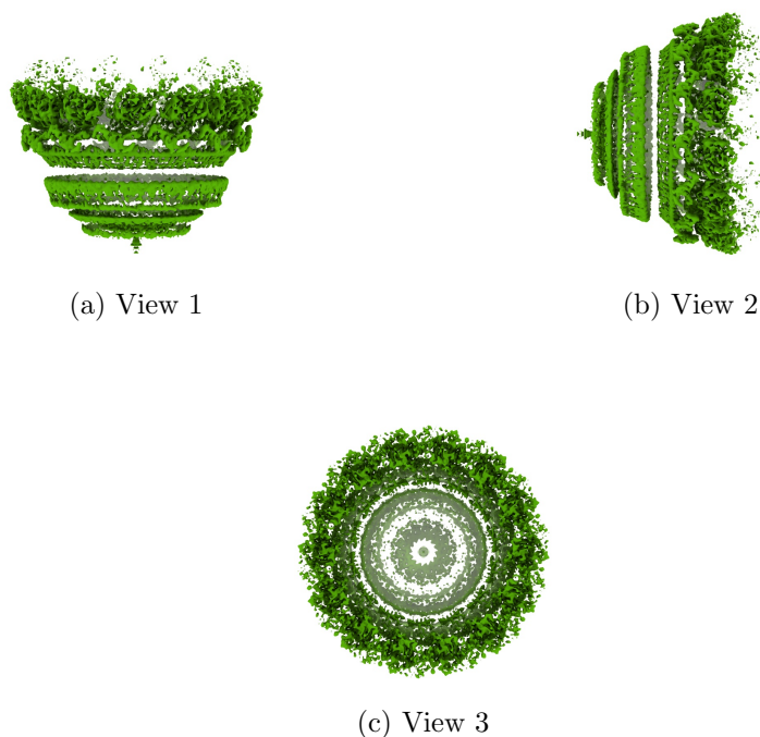
Figure 4: Isosurface at threshold=0.661000. Views generated by ChimeraX at a the following X, Y, Z angles: View 1 (0, -90, -90), View 2 (-90, 0, -90), View 3 (0, 0, 0).
