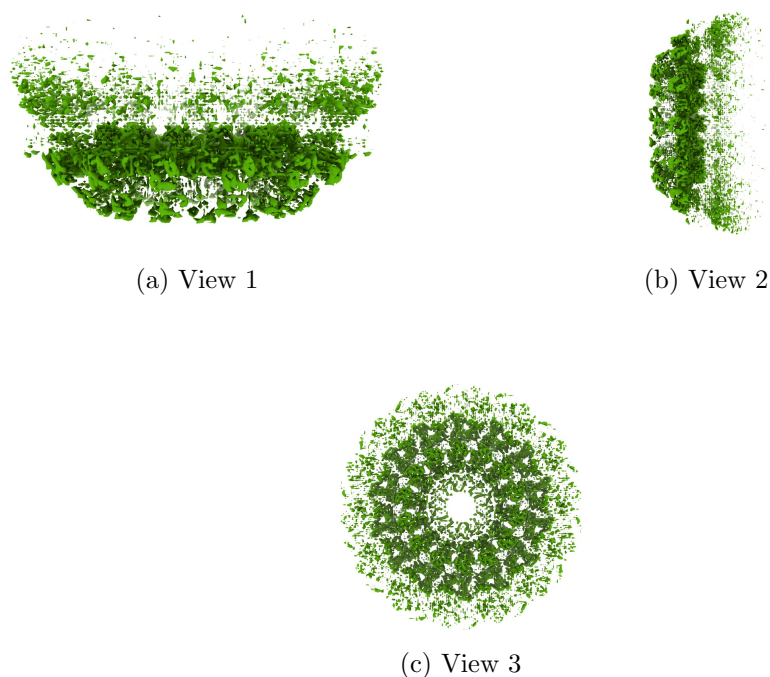
Figure 4: Isosurface at threshold=0.548000. Views generated by ChimeraX at a the following X, Y, Z angles: View 1 (0, -90, -90), View 2 (-90, 0, -90), View 3 (0, 0, 0).
