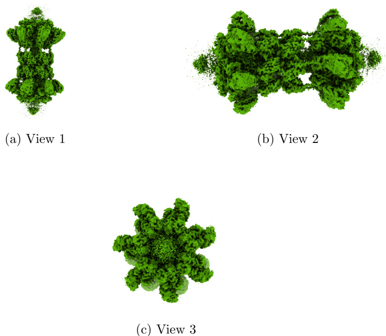
Figure 4: Isosurface at threshold=0.004800. Views generated by ChimeraX at a the following X, Y, Z angles: View 1 (0, -90, -90), View 2 (-90, 0, -90), View 3 (0, 0, 0).
