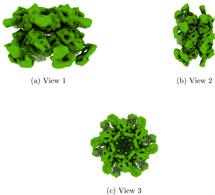
Figure 4: Isosurface at threshold=0.456000. Views generated by ChimeraX at a the following X, Y, Z angles: View 1 (0, -90, -90), View 2 (-90, 0, -90), View 3 (0, 0, 0).
