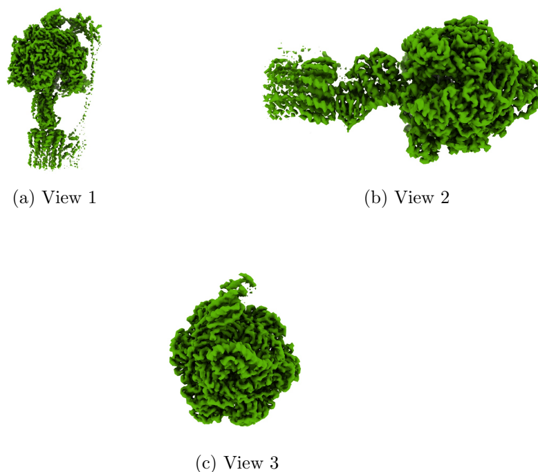
Figure 4: Isosurface at threshold=0.008600. Views generated by ChimeraX at a the following X, Y, Z angles: View 1 (0, -90, -90), View 2 (-90, 0, -90), View 3 (0, 0, 0).
