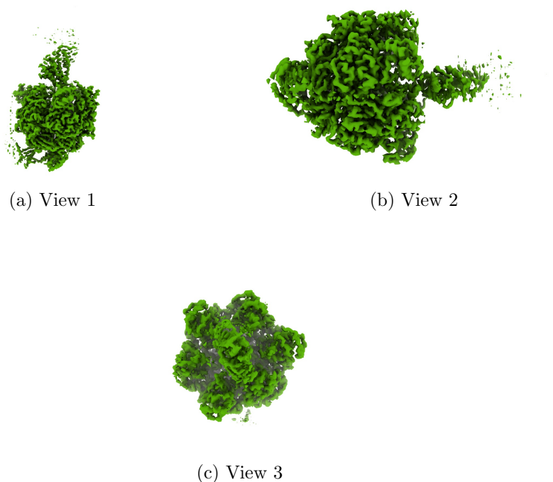
Figure 4: Isosurface at threshold=0.015200. Views generated by ChimeraX at a the following X, Y, Z angles: View 1 (0, -90, -90), View 2 (-90, 0, -90), View 3 (0, 0, 0).
