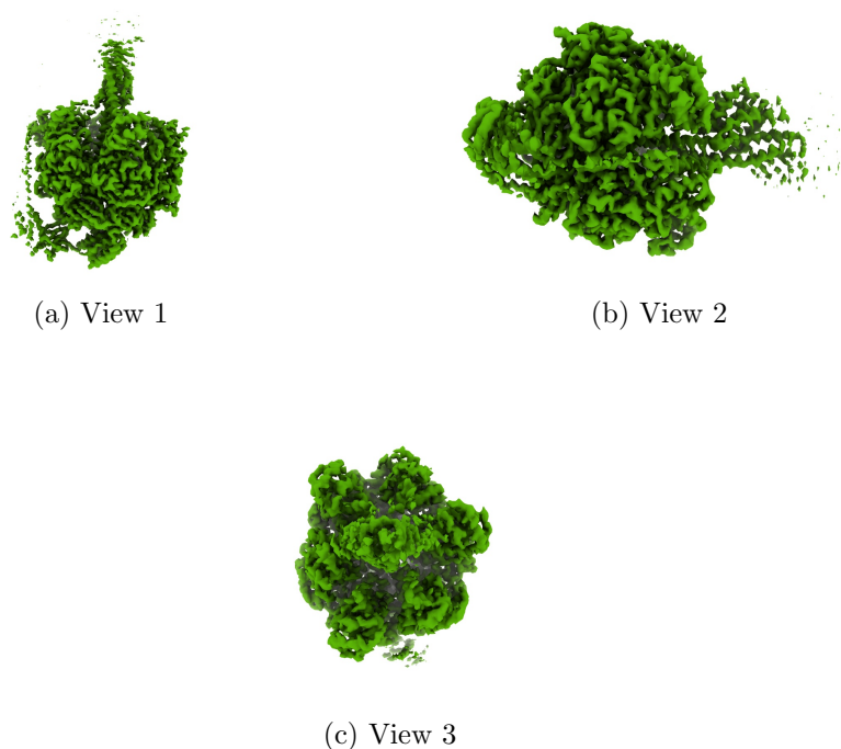
Figure 4: Isosurface at threshold=0.012300. Views generated by ChimeraX at a the following X, Y, Z angles: View 1 (0, -90, -90), View 2 (-90, 0, -90), View 3 (0, 0, 0).
