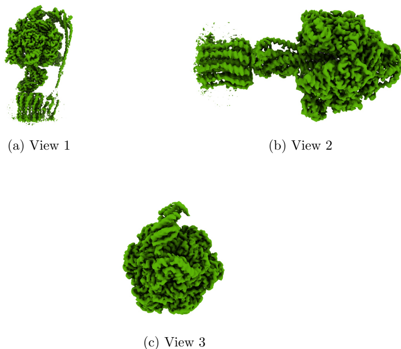
Figure 4: Isosurface at threshold=0.010500. Views generated by ChimeraX at a the following X, Y, Z angles: View 1 (0, -90, -90), View 2 (-90, 0, -90), View 3 (0, 0, 0).
